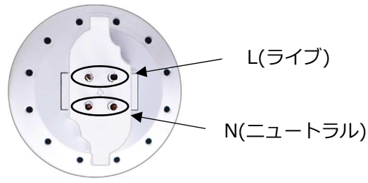
FDL 口金(GX10 q)
